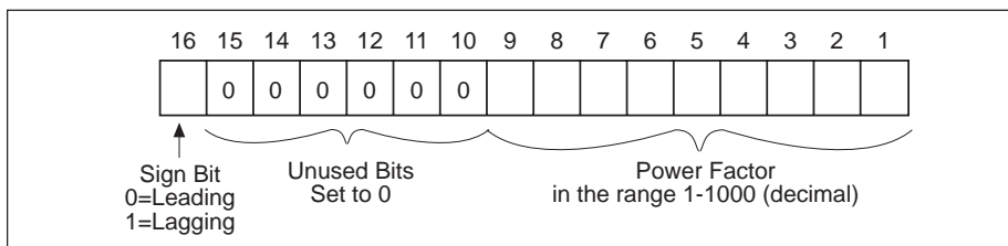
Figure 9-2: Power factor register format
