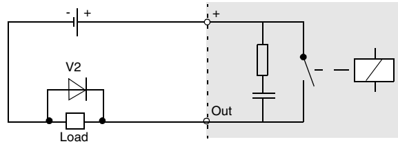
V2 Clamping diode as the protective circuit
