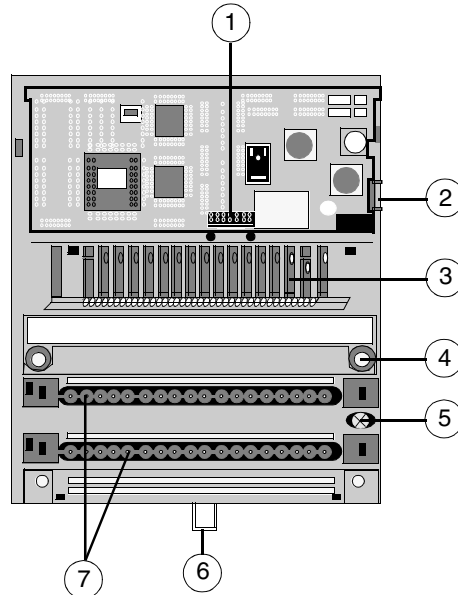
Components of the I/O Module
