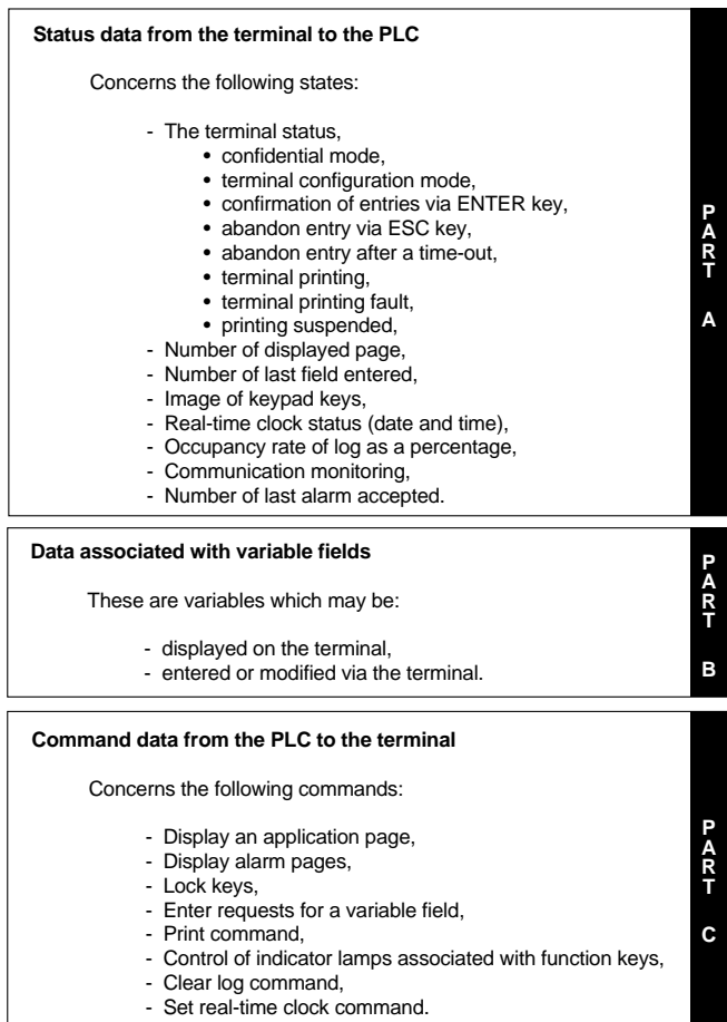
Figure 33: Dialogue Table Structure
