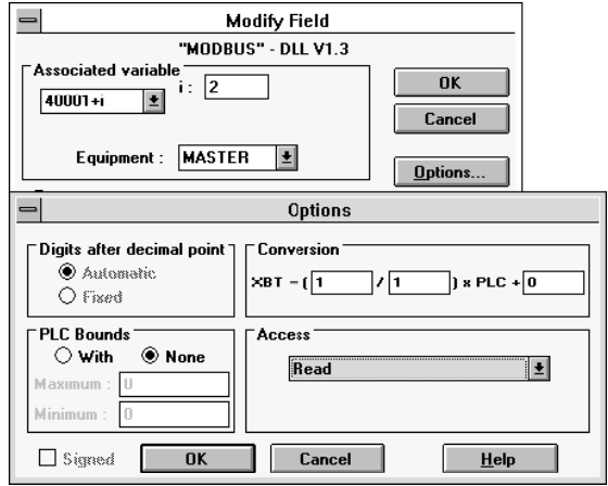
Figure 16: Modify Field Options Window
