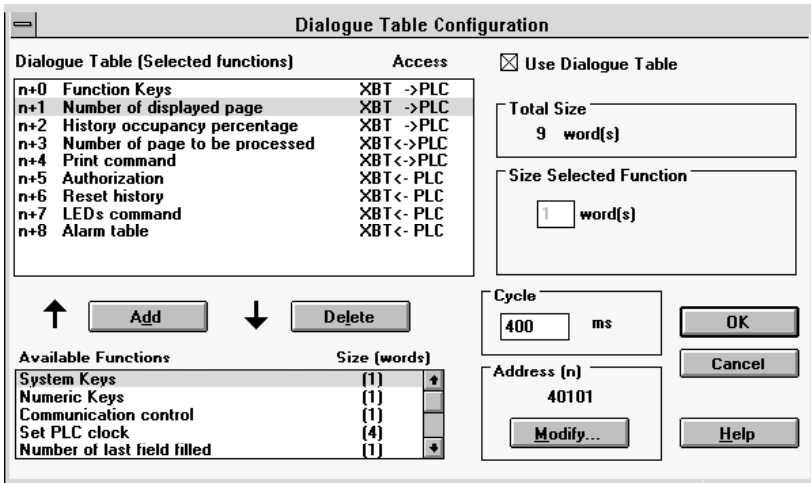
Figure 21: Configuring the Dialogue Table
