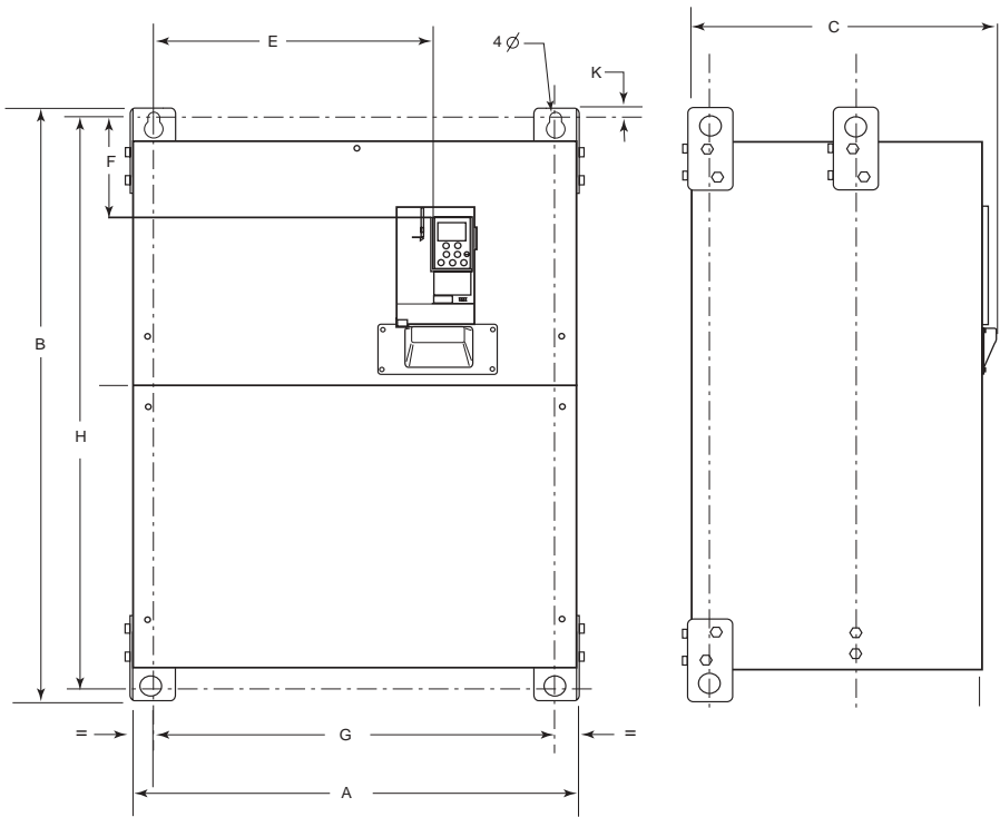
Figure 5: ATV58H Dimensions
