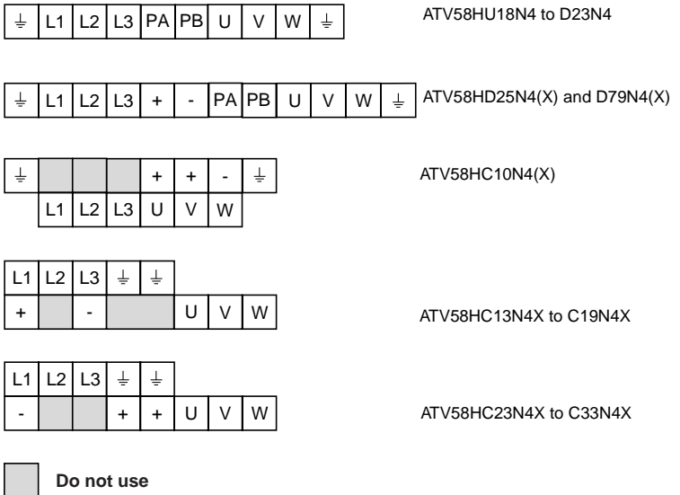
Figure 21: Power Terminal Layout
