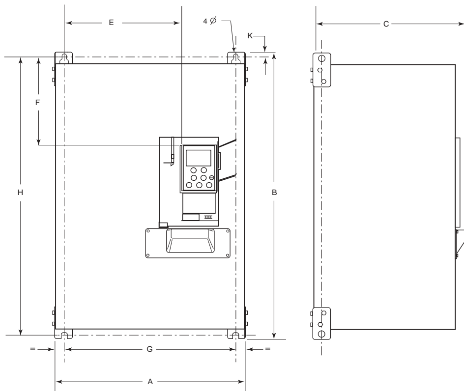
Figure 3: ATV58H Dimensions
